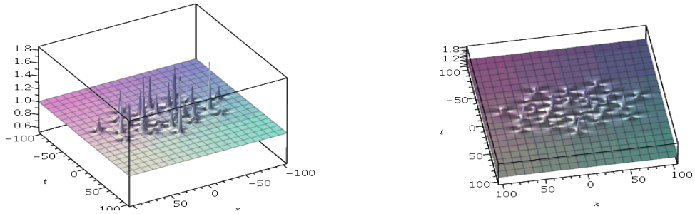
Figure 4: Solution of NLS, N=7 ; \tilde{b}_3 = 10^{10} , 4 rings with 7 peaks on each of them without central peak; on the right, sight of top.
