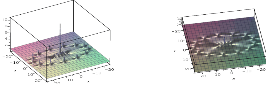
Figure 7: Solution of NLS, N=7 ; \tilde{a}_6 = 10^{12} , \tilde{b}_6 = -10^8 , a ring with 13 peaks and in the center the Peregrine breather of order 5, P_5 ; on the right, sight of top.
