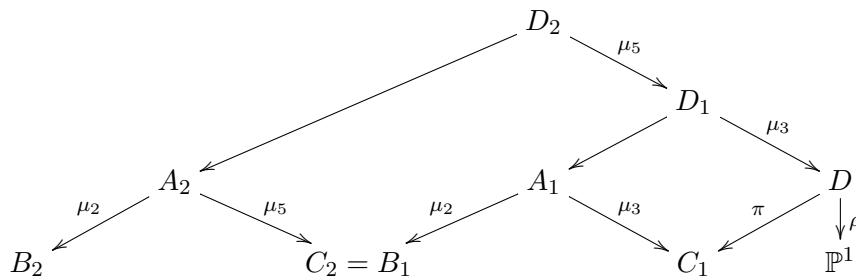
FIGURE 1. Composing parameterizations.
