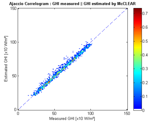
Figure 4 : Scatter density plot of GHI computed by McCclear model in function of ground measurements from Ajaccio. Color bar shows percentage of total samples number.
