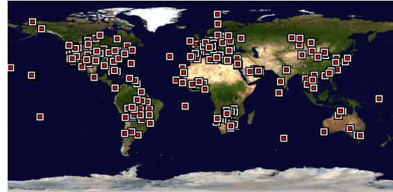
Figure 1: Map of AERONET stations (from NASA)
