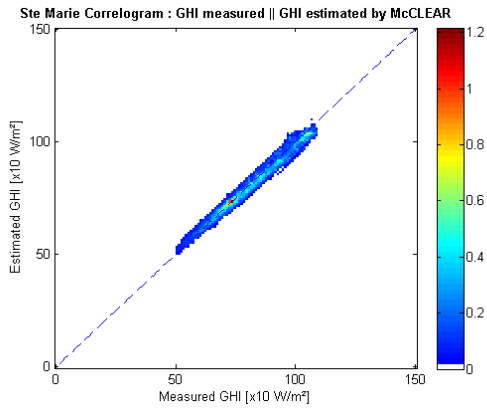
Figure 3: Scatter density plot of GHI computed by McClear model in function of ground measurements from Sainte-Marie. Color bar shows percentage of total samples number.
