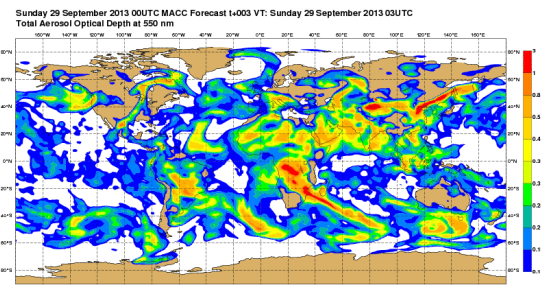
Figure 2: An example of aerosol optical depth map provided by MACC service (from Copernicus)
