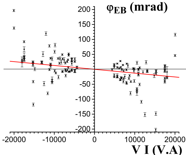
FIG. 12: (color online) Measured values of \varphi_{EB}(V, I) given by eq. (3) as a function of the VI product measured in VA. The (red) full line represents the expected value of the HMW phase, \varphi_{HMW}(V, I) = -(1.28 \pm 0.03) \times 10^{-6}VI rad.
