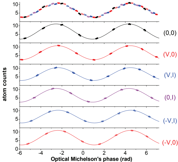
FIG. 3: (color online) Recorded data with 6 (V, I) configurations during a single fringe scan: the number of detected atoms per second (the unit is 10^4 detected atoms/second and the counting period is 0.1 second) is plotted as a function of the phase of the optical Michelson interferometer which directly maps the position x_3 of mirror M_3 . The signals corresponding to different field configurations are plotted with different symbols: black squares for (0, 0) , red bullets for (V, 0) , blue full triangle for (V, I) , open violet squares for (0, I) , open blue triangle for (-V, I) and open red circles for (-V, 0) . The top graph represents the signal as it is recorded and the signal corresponding to each one of the 6 (V, I) configurations is plotted separately below with its best fit.
