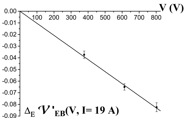
FIG. 14: Plot of difference of visibility for opposite V values, \Delta_E \mathcal{V}'_{EB}(V, I = 19 \text{ A}) , as a function of V . The current value I = 19 \text{ A} , chosen close to the cancelation of D_0 = \sum \cos(\phi_Z) , enhances the sensitivity of the visibility to the AC phase. The measured values (squares) are well represented by a linear function of V , as predicted by our model.
