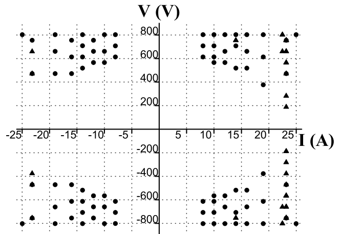
FIG. 11: Data set collected for the measurement of the HMW phase. Each run is represented in the I, V plane by a triangle (respectively a bullet) for a 4-field (respectively 6-field) experiment.
