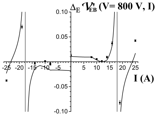
FIG. 13: Plot of \Delta_E \mathcal{V}'_{EB}(V = 800 \text{ V}, I) as a function of the current I : the measured data points (squares) are compared to the result of our model (full line). The visibility, proportional to D_0 = \sum \cos(\phi_Z) vanishes when I \approx \pm 18 \text{ A} indicated by vertical lines: this induces a divergence of the prediction of our model, which uses a first-order calculation in D_{\pm, \pm}/D_0 . Our model explains well the main variations of \Delta_E \mathcal{V}'_{EB}(V, I) , even if some imperfections appear clearly.
