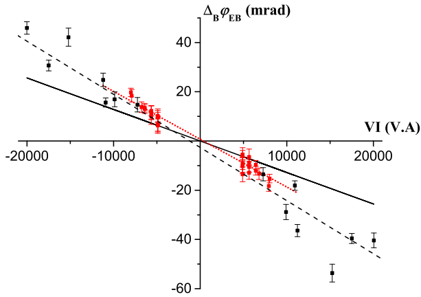
FIG. 19: (color online) Measured values of \Delta_B \varphi_{EB}(V, I) as a function of the VI product. The data points with |I| \leq 12 A are plotted in red as well as their fit represented by a dotted line. The data points with |I| > 12 A are plotted in black as well as their fit represented by a dashed line. The expected dependence of \varphi_{HMW}(V, I) with the VI product is represented by a black full line.
