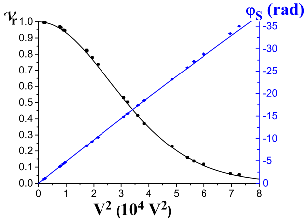
FIG. 4: (color online) The relative visibility \mathcal{V}_r (left scale, black squares and line) and the fringe phase shift \varphi_S (rad) (right scale, blue bullets and line) are plotted as a function of V^2 , where V is the voltage applied to one capacitor only. The points are experimental and the curves are their best fits.
