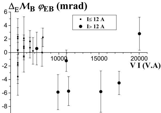
FIG. 17: Plot of the quantity \Delta_E \mathcal{M}_B \varphi_{EB}(V, I) as a function of the VI product: different symbols depending if |I| \leq 12 A or |I| > 12 A.
