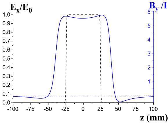
FIG. 2: (color online) Calculated components E_x (dashed line) and B_y (full line) as a function of z in the interaction region. For the electric field, the plotted quantity is E_x/E_0 , where E_0 = V/h is the field of an infinite plane capacitor, with a spacing h and an applied voltage V . For the magnetic field, the plotted quantity B_y/I , where I is the coil current, is in units of 10^{-4} T/A.
