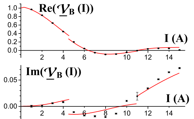
FIG. 9: (color online) Real and imaginary part of the complex fringe visibility as a function of the HMW coil current I (note the expanded scale for \text{Im}(\mathcal{V}_B(I)) ). The points are experimental and the curves are the results of best fits, with 3 different \chi values: \chi = 0.077 for I = 0 - 4 A; \chi = -0.014 for I = 5 - 10 A; \chi = -0.062 for I = 11 - 15 A. When these experiments were done, we had not understood that the laser frequency must be tightly controlled in order to keep \chi very small and this explains why large \chi values are observed. We get A_{J1} = -0.46 \pm 0.02 rad/A; A_{J2} = (-110 \pm 8) \times 10^{-4} rad/A ^2 ; A_{J3} = (-20 \pm 4) \times 10^{-5} rad/A ^3 ; I_0 = 0.32 \pm 0.05 A and J_{0,I} = -0.55 \pm 0.13 rad.
