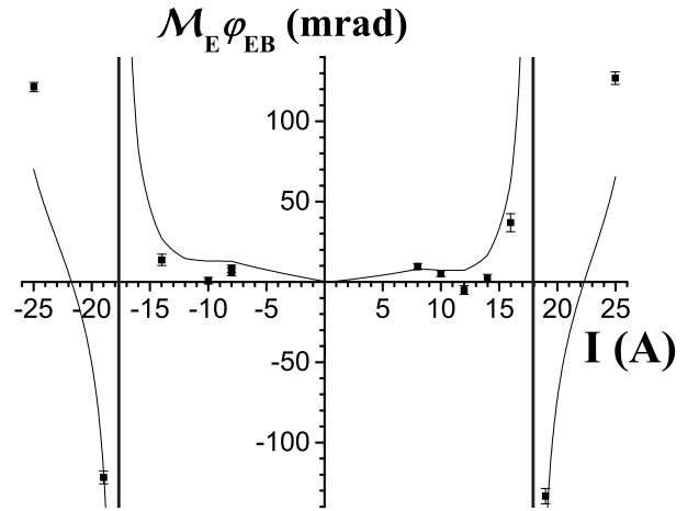
FIG. 18: Plot of the quantity \mathcal{M}_E \varphi_{EB}(V, I) for V = 800 V, as a function of the current I . The points are measured values, the line is a best fit for all the measurements of \mathcal{M}_E \varphi_{EB} (see discussion). As for fig. 13, vertical gray lines indicate cancellation of the visibility.
