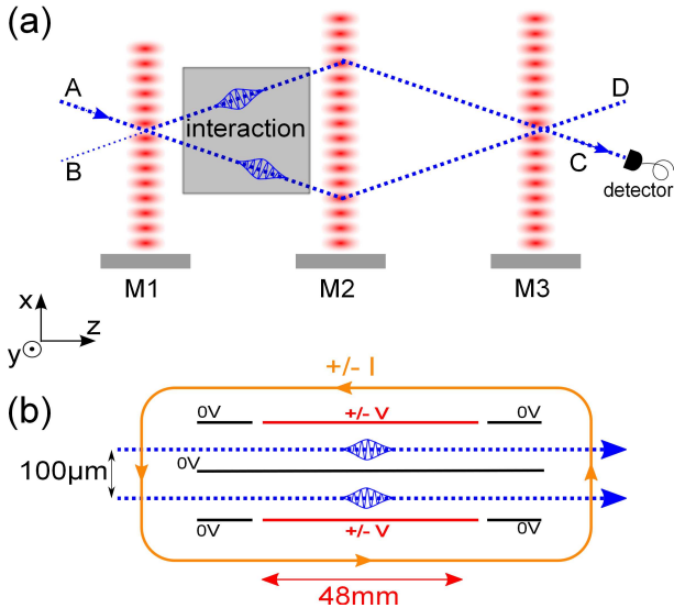
FIG. 1: (color online) Schematic top views (not to scale) of our atom interferometer (panel a) and the interaction region for the observation of the HMW phase (panel b). Our atom interferometer is a Mach-Zehnder interferometer, with two entrances A and B (only A is used) and two exits C and D (C is detected). An atomic beam (dotted blue lines) entering by A is diffracted by three quasi-resonant laser standing waves produced by the mirrors M_i . The largest distance between interferometer arms, about 100 \mu\text{m} , occurs just before the second laser standing wave, where we introduce the interaction region. The opposite electric fields necessary for the observation of the HMW phase are horizontal. They are produced by two plane capacitors (high voltage electrodes in red; grounded electrodes in black). The septum is a thin common electrode located between the two interferometer arms represented by dotted blue lines. Two rectangular coils (represented by the brown rectangle) produce the vertical magnetic field.
