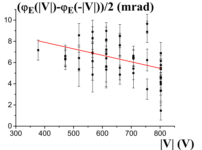
FIG. 6: (color online) Fringe phase shifts induced by electric fields applied to both capacitors: the difference quantity (\varphi_E(|V|) - \varphi_E(-|V|))/2 is plotted as a function of |V| . The points are experimental and the straight line is the best linear fit.
