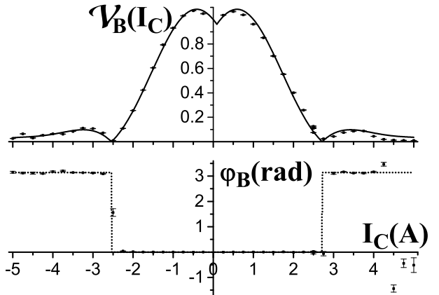
FIG. 8: Relative visibility (upper panel) and phase shift (lower panel) as a function of the compensator current I_C (A). The points are experimental and the curves represent their best fit, with A_{J1,C} = 1.52 \pm 0.02 rad/A, I_{0,C} = 0.09 \pm 0.02 A and J_{0,C} = -0.63 \pm 0.03 rad. The minor deviations which appear when I_C > 4 A are probably due to the arbitrary assumption of balanced sublevel populations ( \chi = 0 ) for this particular example.
