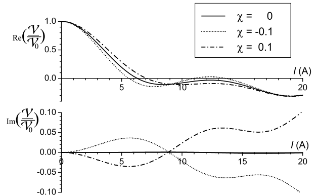
FIG. 7: Calculated real and imaginary parts of the complex visibility \underline{\mathcal{V}}/\mathcal{V}_0 as a function of the coil current I . We use the values J_1/I = 0.5 rad/A and J_2/I^2 = 0.01 rad/A 2 , which are close to our experimental values. Same S_{||} and \chi values as in fig. 6.
