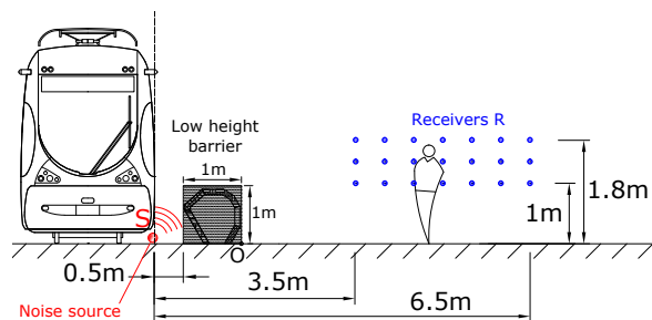
Figure 2 - Geometrical configuration for the implementation of the low-height tramway noise barrier. Dotted line: idealization of the tramway side as a vertical baffle.
