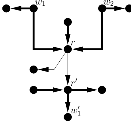
Figure 4: The collecting gadget \overrightarrow{G^r} , and a locally irregular 2-arc-colouring of \overrightarrow{G^r} (thick (resp. thin) arcs are arcs coloured 1 (resp. 2)).
