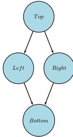
Fig. 3: The diamond-shaped G-ACG \mathcal{D} .
