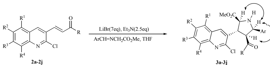
Scheme 2. Synthesis of quinolylypyrrolidine N-H derivatives ( 3a-3j ).
