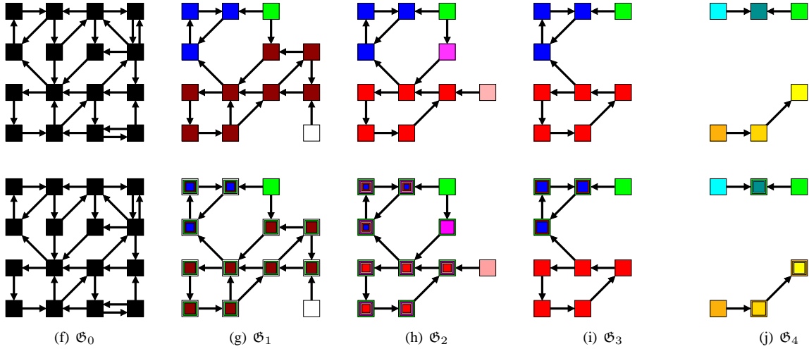
Fig. 5. A stack \mathcal{S} = (\mathfrak{G}_0, \mathfrak{G}_1, \mathfrak{G}_2, \mathfrak{G}_3, \mathfrak{G}_4) . First row: Each color represents a S-component. Second row: Each color represents a D-component (vertices with more than one color belong to all the associated D-components).
