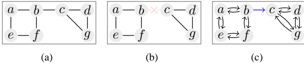
Fig. 2. Undirected and directed graphs (see text).
