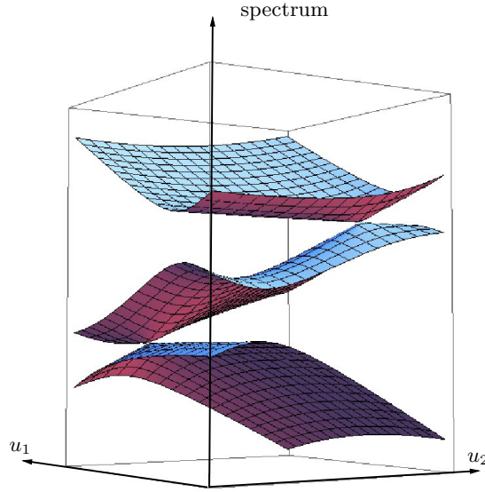
Figure 2: A conically connected spectrum in the case m = 2 .
