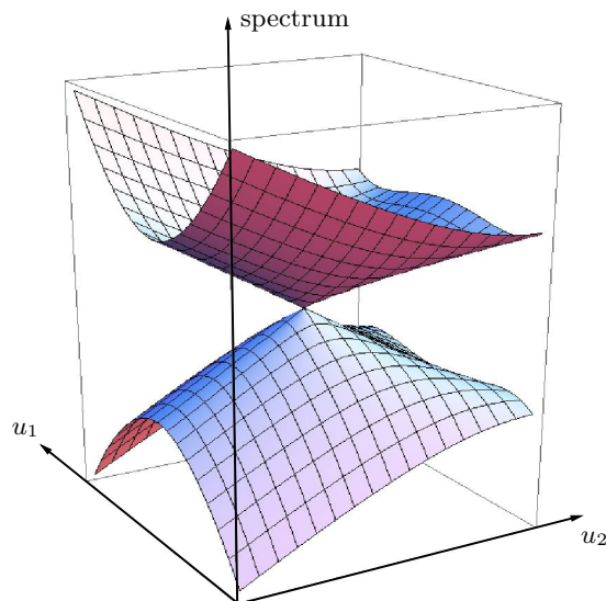
Figure 1: A conical intersection when m = 2 : the surfaces represent two eigenvalues of H(u_1, u_2) as functions of u_1 and u_2 .
