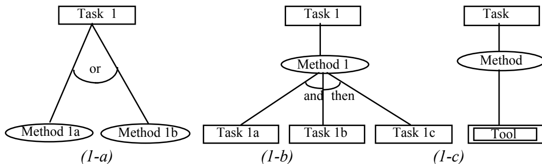
Figure 1: Various possible organizations of tasks, methods and tools (1-a): Several methods can be associated to a task (1-b): Task / sub task decomposition (complex method) (1-c): Method calling a tool (terminal method).
