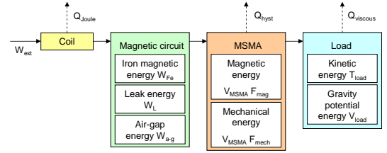
Fig. 4. Example of a simple MSMA based actuator: partition of the different energy contributions, Gauthier et al. (2008).
