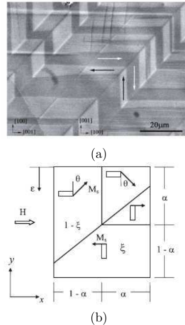
Fig. 8. Internal variables and cristallographic microstructure of NiMnGa MSMA: (a) Image of twin-variant NiMnGa microstructure by scanning electron microscope, (b) Simplified two-variant microstructure of NiMnGa (Representative Volume Element). Sarawate and Dapino (2010).
