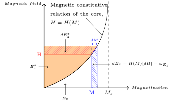
Fig. 5. Zeeman magnetic energy density stored in the core of a magnetic circuit (iron magnetization energy).
