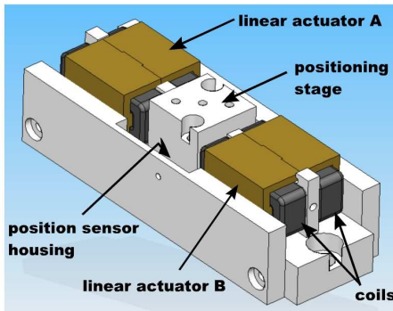
Fig. 2. CAD model of the push-pull actuator using two antagonist MSMA samples in Hubert et al. (2012).
