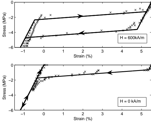
Fig. 7. Mechanical stress versus strain curves with and without magnetic field for a cyclic charging (simulation: solid line, experimental results: cross points), Gauthier et al. (2008).
