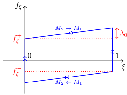
Fig. 9. Exemple of constitutive law for irreversible internal state variable: coordinate \xi versus dual internal force f_\xi , Gauthier et al. (2008).
