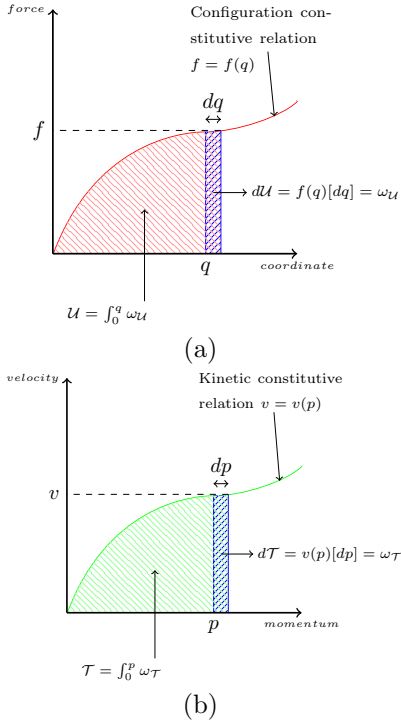
Fig. 3. Graphical links between dual, state variables, system behaviour and state functions as exact linear differential 1-form: (a) Static/configuration behaviour, (b) kinetic behaviour.
