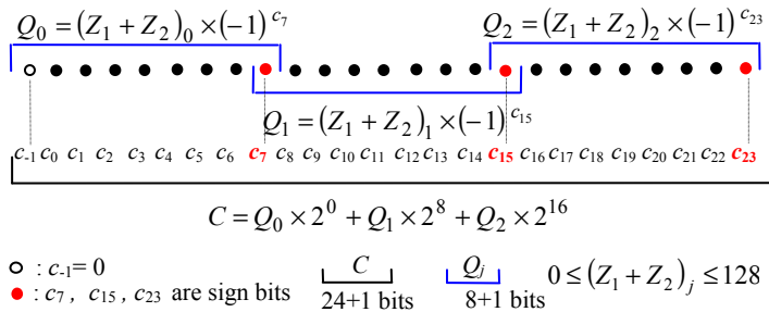
Figure 1. Partitioning of a 24-bit C constant using R3 algorithm.
