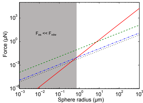
Fig. 4. Van der Waals (green dashed line) force, electrostatic force F_{es} induced by tribo-electrification (red solid line) and maximal electrostatic force F_{VF} induced by contact electrification (black dashed line) calculated between a sphere and a plane according to the sphere radius. The electrostatic force F_{VF} induced by contact electrification appears negligible. The electrostatic force F_{es} is considered as negligible as it is lower than the tenth of the van der Waals forces (blue dash-dot line). Considered materials for van der Waals and F_{es} calculations are borosilicate glass, with A_{12} = 6.5 \times 10^{-20} \text{ J} , z_0 = 0.3 \text{ nm} and \sigma = 0.15 \text{ mC.m}^{-2} .
