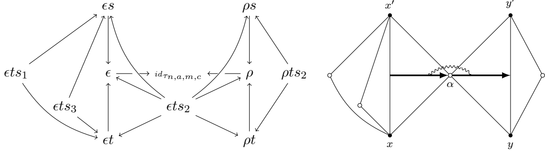
Figure 3: Category of elements for \tau_{2,1,3,2} and graphical representation
