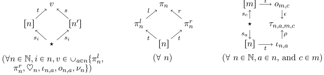
Figure 2: Equations for \mathbb{C}
