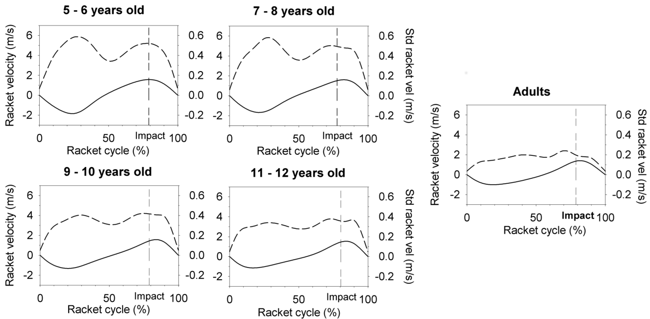
Figure 5. Racket velocity profiles. Mean racket velocity (solid line) and mean within-trial standard deviation (dash line) for the last trial of each age group.
