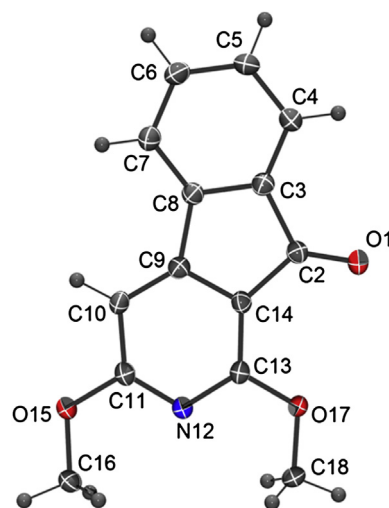
Fig. 3. ORTEP diagram (50% probability) of compound 24 .
