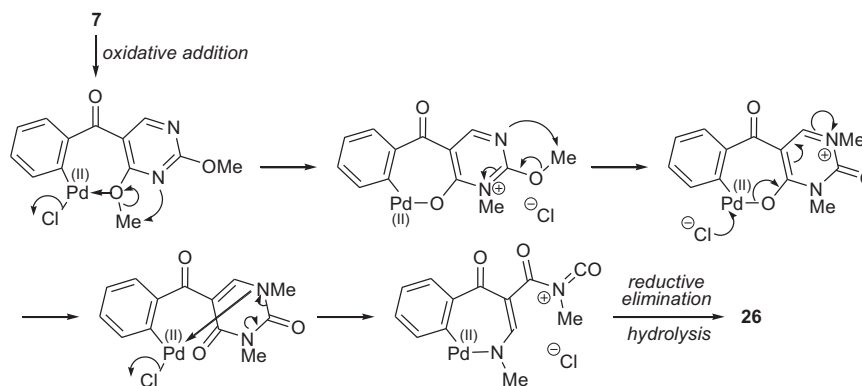
Scheme 7. Mechanistic sequence proposed for the formation of 26 .
