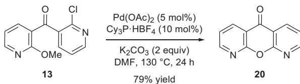
Scheme 3. Synthesis of 5 H -pyrano[2,3- b :6,5- b' ]dipyridin-5-one ( 20 ) from 13 .
