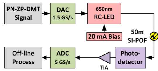
Fig. 4: Experimental system setup
