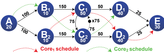
Fig. 2. Single-rate SDF (Directed Acyclic Graph if dotpoint FIFO is ignored) Dotpoint arrows depict new precedence relationships introduced by a schedule of the DAG on an architecture with 2 cores.
