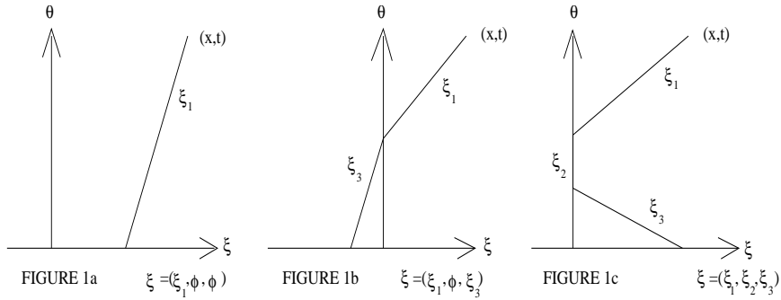
Figure 1: Characteristic curves
