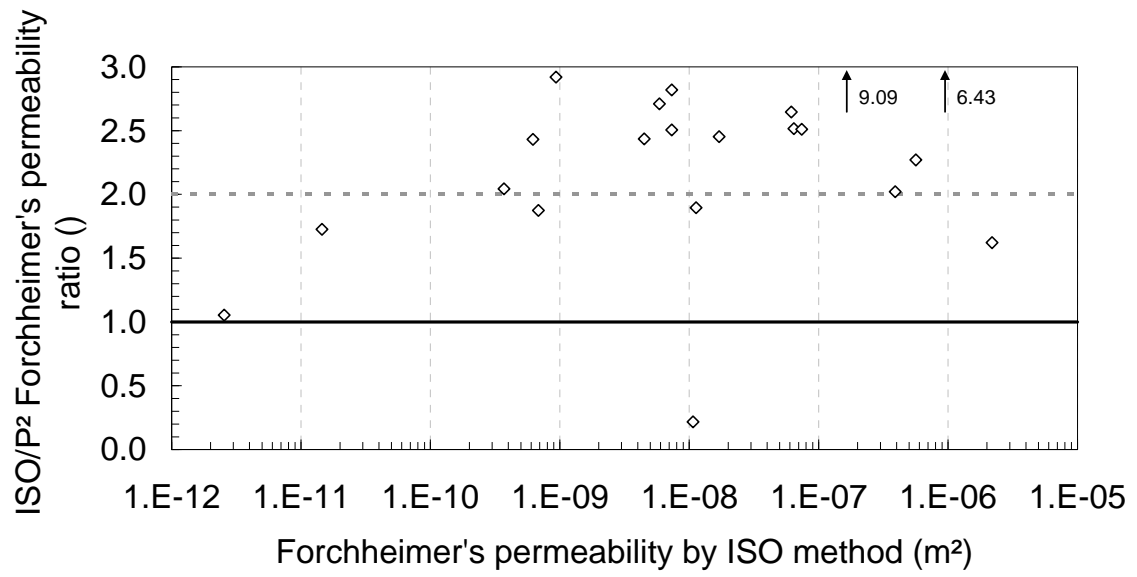
Figure 7. Ratio of Forchheimer's term found with each method.
