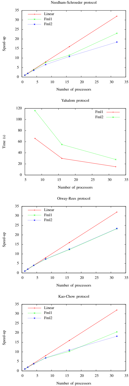
Figure 7. Benchmark results for the four protocols where Fml1 is “secrecy” and Fml2 ‘aliveness’”
