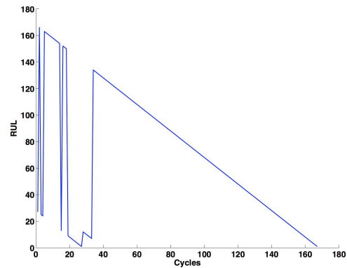
Figure 7: Estimated RUL for B0007.
