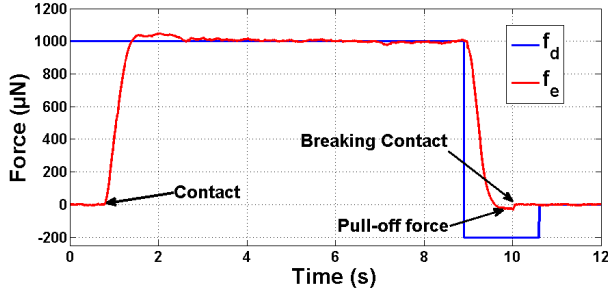
FIGURE 12. THE PULL-OFF FORCE APPEARS WHILE BREAKING THE CONTACT. EXPERIMENT DONE FOR IMPEDANCE CONTROL SCHEME
