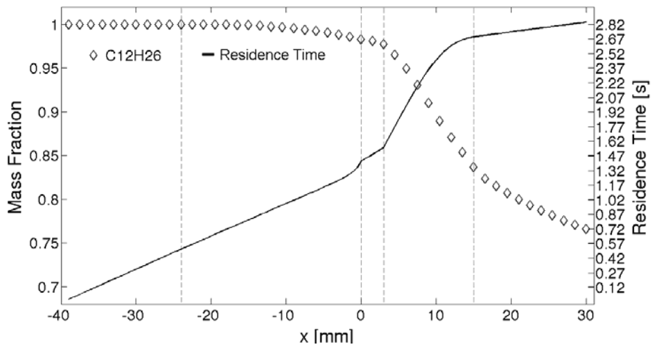
5 Figure 12. Dodecane mass fraction inside the system for case 1 (a) and case 4 (b) with 6 residence time and mass fraction distribution along the symmetric x-axis (c). 7 8
