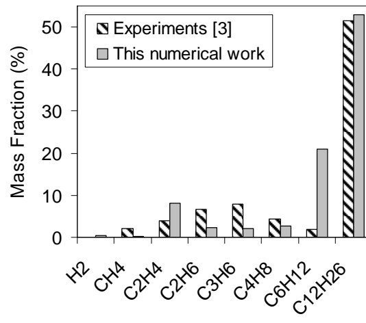
Figure 9. Comparison of the pyrolysis products composition computed for case 1 and measured experimentally in the HPC (a), inside the porous zone (b) and at the process outlet (c).
