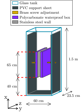
Figure 2: Drawing of the experimental apparatus.
