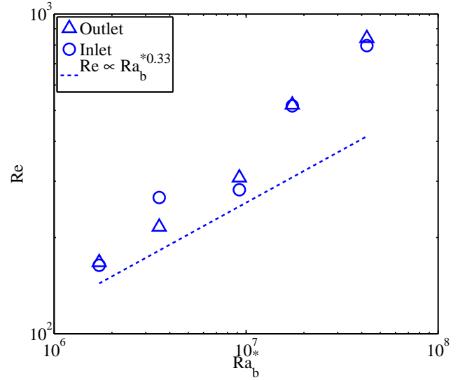
Figure 14: Reynolds number versus modified Rayleigh number for the five experiments, calculated at the channel outlet (traingles) and at the inlet (rounds).
