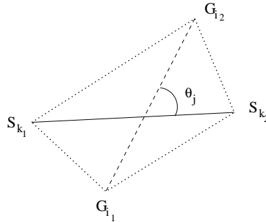
Figure 6: Angle between diagonals of a diamond cell.
