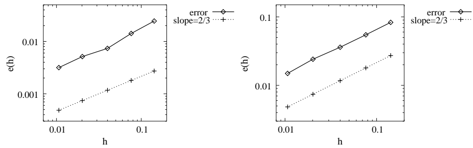
Figure 7: Unstructured meshes.
