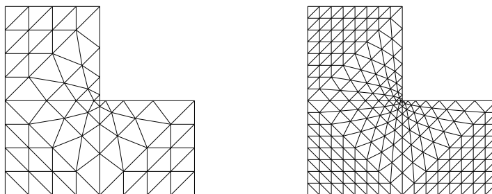
Figure 10: \alpha -refined meshes with n=4 and n=8 .
