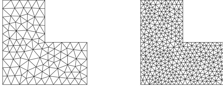
Figure 7: Unstructured meshes.
