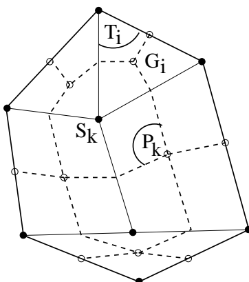
Figure 2: An example of a primal mesh and its associated dual mesh.
