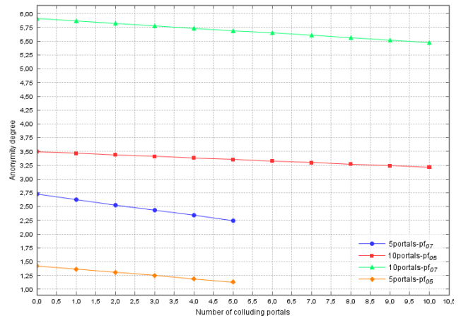
Figure 3. Anonymity degree
