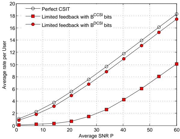
Fig. 4: Average rate per user versus the average SNR P in the distributed CSIT scenario with B = B^{\text{CCSI}} (Cf. (15)) and B = B^{\text{DCSI}} (Cf. (18)) for b = 5 + 4 \log(K) , compared to the average rate per user obtained with perfect CSIT.
