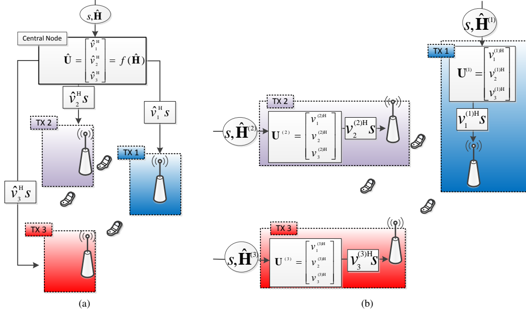
Fig. 1: The transmission with centralized CSIT/precoding is symbolically represented in Figure (a) while Figure (b) represents the distributed CSIT/precoding .
