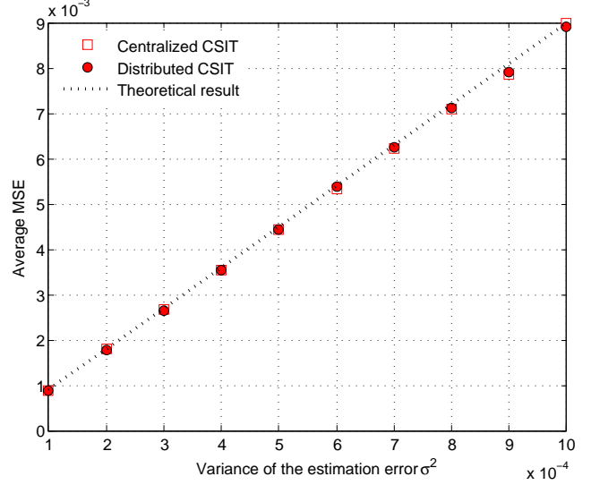
Fig. 2: Average MSE \mathbb{E}[\|\mathbf{u}_i^{(j)} - \mathbf{u}_i^*\|^2] (resp. \mathbb{E}[\|\mathbf{u}_i^{\text{CCSI}} - \mathbf{u}_i^*\|^2] ) as a function of \sigma^2 .
