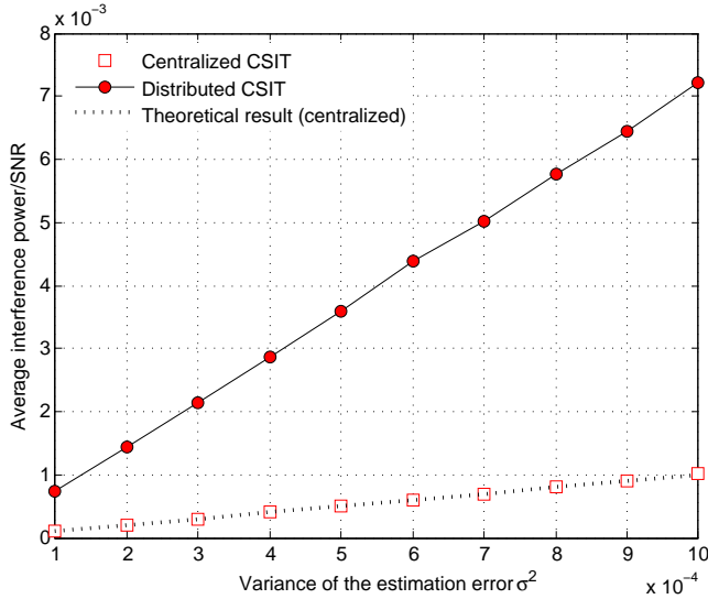
Fig. 3: Average value of the leaked interference after normalization by the average SNR E[|\mathbf{h}_i^H \mathbf{u}_j^{\text{DCSI}}|^2] (resp. E[|\mathbf{h}_i^H \mathbf{u}_j^{\text{CCSI}}|^2] ) as a function of \sigma^2 .
