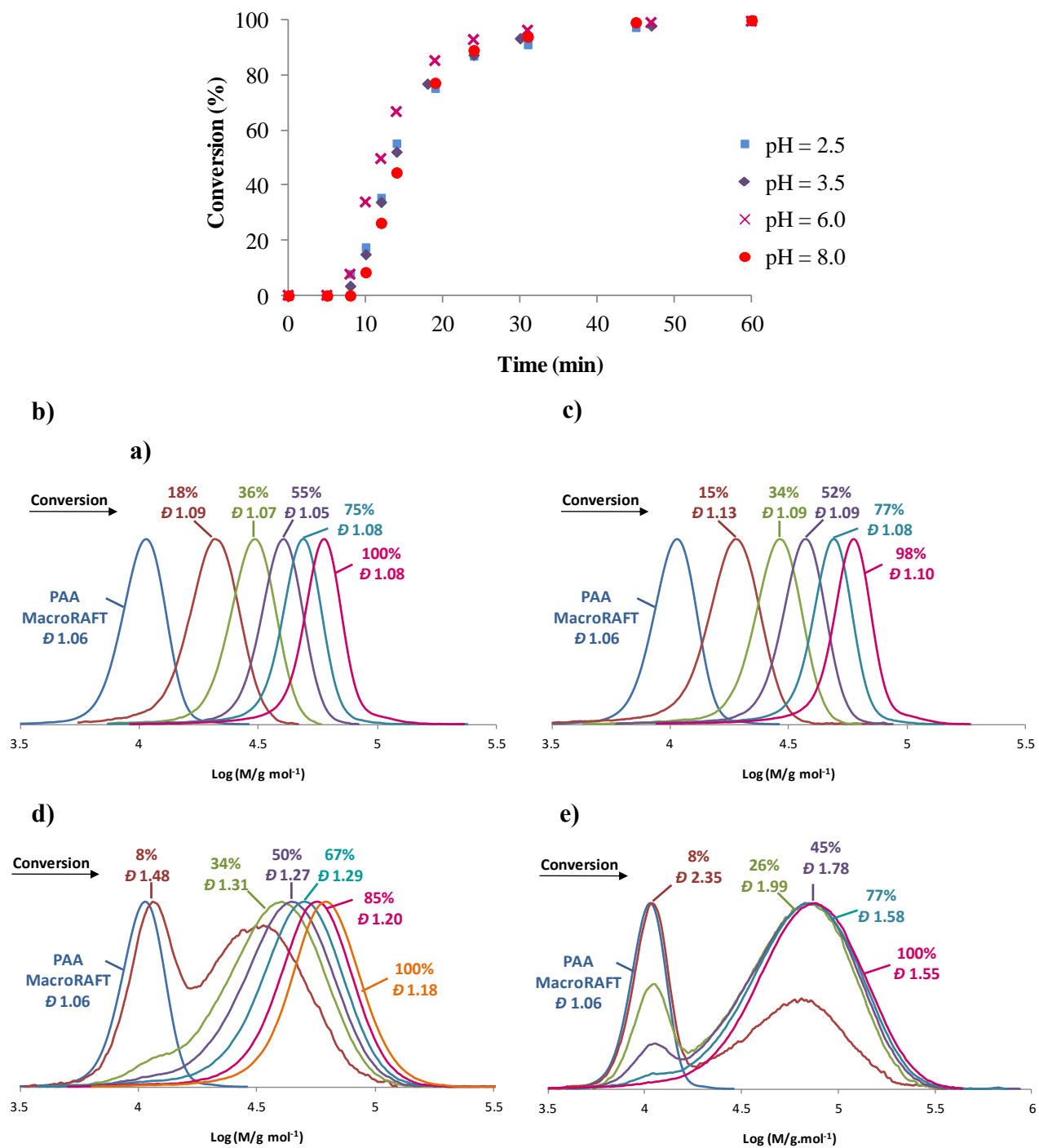
Figure 6: Chain extension experiments of PAA-CTPPA ( M_n = 4480 \text{ g mol}^{-1} , \bar{D} = 1.11 ) with NAM at different pHs at 80 °C. [\text{NAM}]/[\text{PAA}] = 400 , [\text{CTPPA}]/[\text{ACPA}] = 10 . Evolution of (a) monomer conversion versus time. Corresponding SEC chromatogram evolutions for (b) pH = 2.5, (c) pH = 3.5, (d) pH = 6.0 and (e) pH = 8.0.
