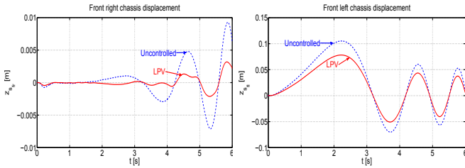
Fig. 10. Front right chassis displacement z_{s_{fr}} . Fig. 11. Front left chassis displacement z_{s_{fl}} .
