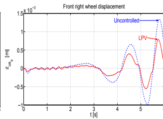
Fig. 23. Front right wheel displacement z_{us_{fr}} .
