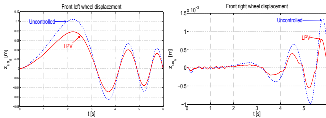
Fig. 22. Front left wheel displacement z_{us_{fl}} .
