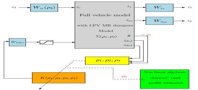
Fig. 5. Suspension control design scheme.
