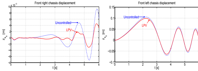
Fig. 18. Front right chassis displacement z_{s_{fr}} .
