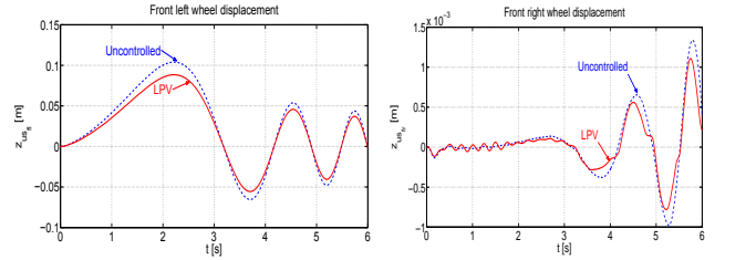
Fig. 14. Front left wheel displacement z_{us_{fl}} . Fig. 15. Front right wheel displacement z_{us_{fr}} .
