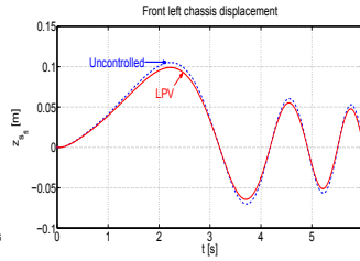
Fig. 19. Front left chassis displacement z_{s_{fl}} .
