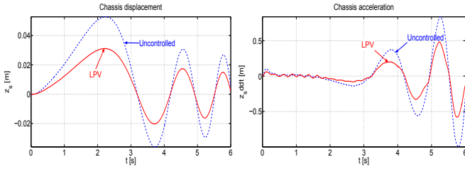
Fig. 8. Chassis displacement of the gravity center z_s . Fig. 9. Chassis acceleration of the gravity center \ddot{z}_s .
