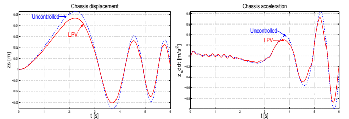
Fig. 16. Chassis displacement of the gravity center z_s . Fig. 17. Chassis acceleration of the gravity center \ddot{z}_s .
