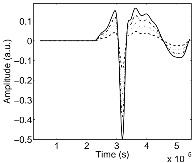
Figure 2. Comparison of signals propagating through the fractal porous medium, for d = 0.2 (solid line), d = 0.4 (dashdot line), d = 0.6 (dotted line) and d = 0.8 (dashed line)
