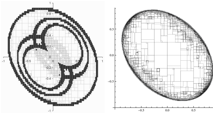
Fig. 4 Pavings for the S&P 2,3,2 problems computed by the method presented in [6] (left) and by our method (right).
