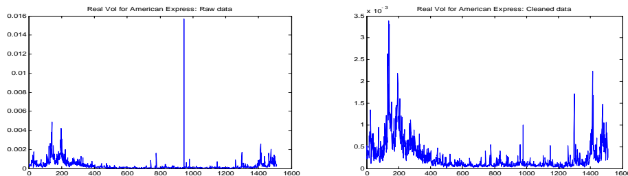
Figure 2: Impact of the cleaning rule on the data. Left: realized volatility for r_{t,j}^{OLD} . Right: realized volatility for r_{t,j}^{NEW} .
