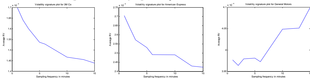
Figure 3: Volatility signature plots for selected stocks.
