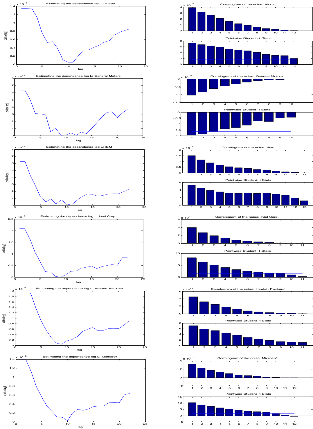
Figure 4: Estimation of MA(L) noise. Left: plot of \Delta(l) against l . The minimum of \Delta(l) is used as the first guess of L . Right: The correlogram of the noise (top) and the associated Student-t (bottom). The line crossing the student-t stats indicates the significance threshold, one-sided, 5%.
