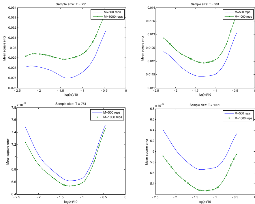
Figure 1: MSE curves of the CGMM estimator for different M and T .
