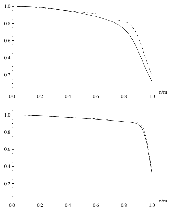
Figure 4: Numerical evaluation of the theoretical (plain) and approached (dashed) probability P_{25,n,15,3,9} for m = 25 (top) or 50 (bottom), and for n varying from 1 to m .
