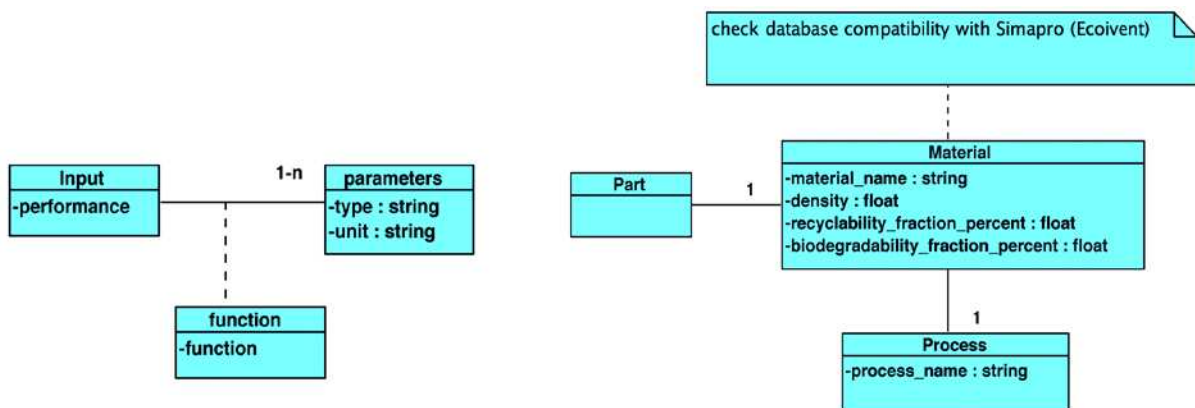
Figure 3: Class diagram of CES Inputs (left) and Outputs (right)
