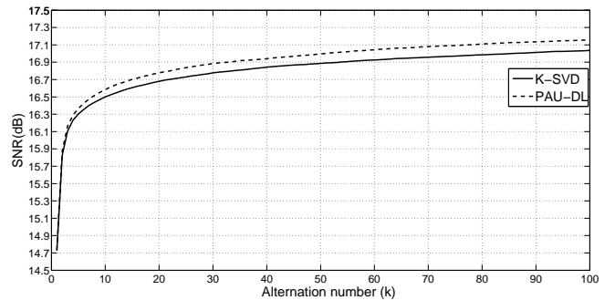
Fig. 3. SNR in dB is plotted versus the alternation number during the learning process.
