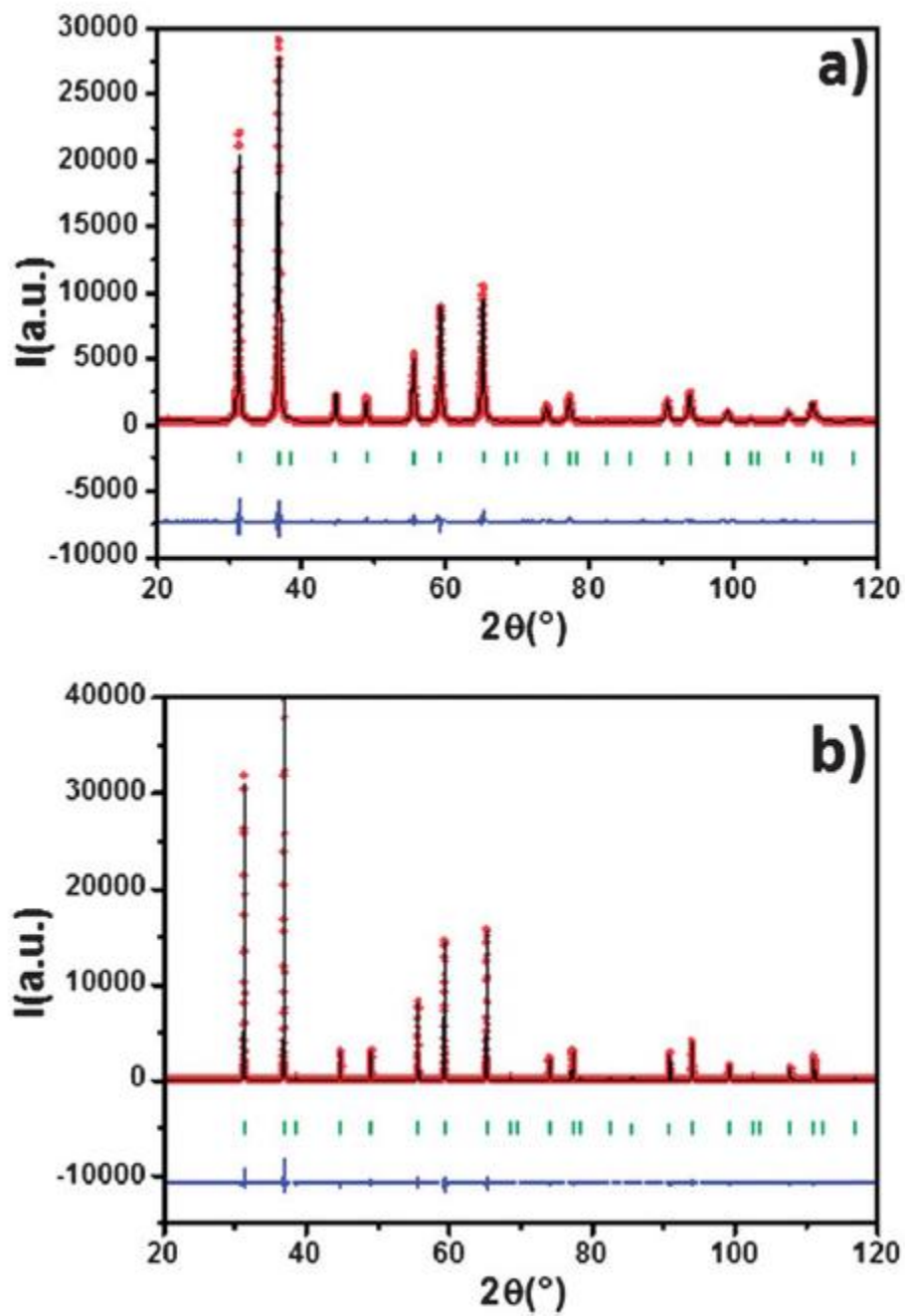
Fig. 4 Refined diffractograms for (a) Pechini 600 °C, (b) Pechini 1200 °C (green tick: theoretical diffraction peak of \text{ZnAl}_2\text{O}_4 ).
