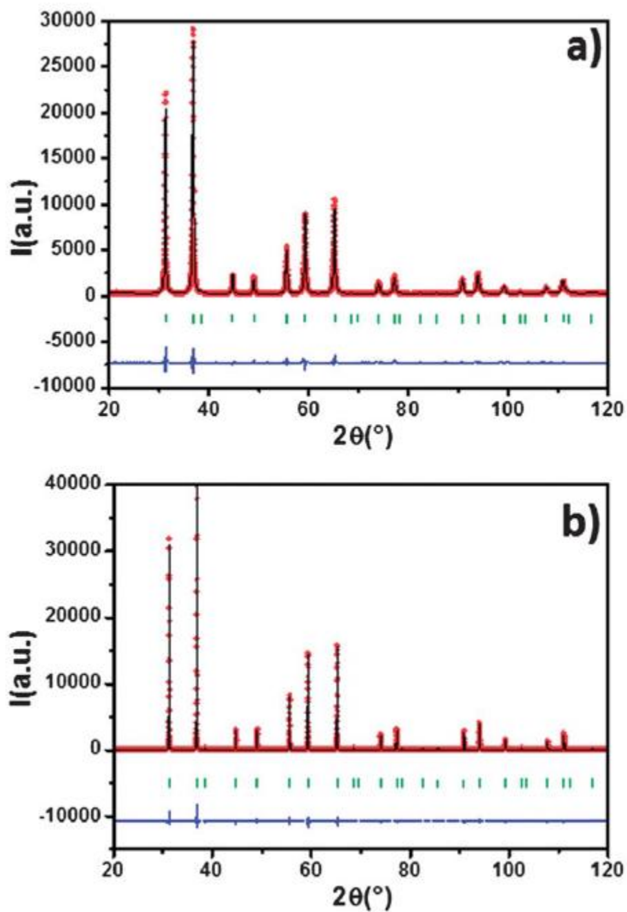
Fig. 4 Refined diffractograms for (a) Pechini 600 ^\circ C , (b) Pechini 1200 ^\circ C (green tick: theoretical diffraction peak of ZnAl_2O_4 ).
