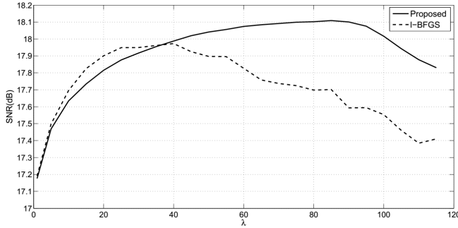
Fig. 2. The final SNR as a function of \lambda in our algorithm and the l-BFGS algorithm.
