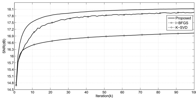
Fig. 3. Results of the experiment on AR(1) signal. SNR is plotted as a function of the alternation number, k , during the learning process. The regularization parameter for our algorithm and the l-BFGS algorithm is \lambda = 85 , and \lambda = 40 , respectively.
