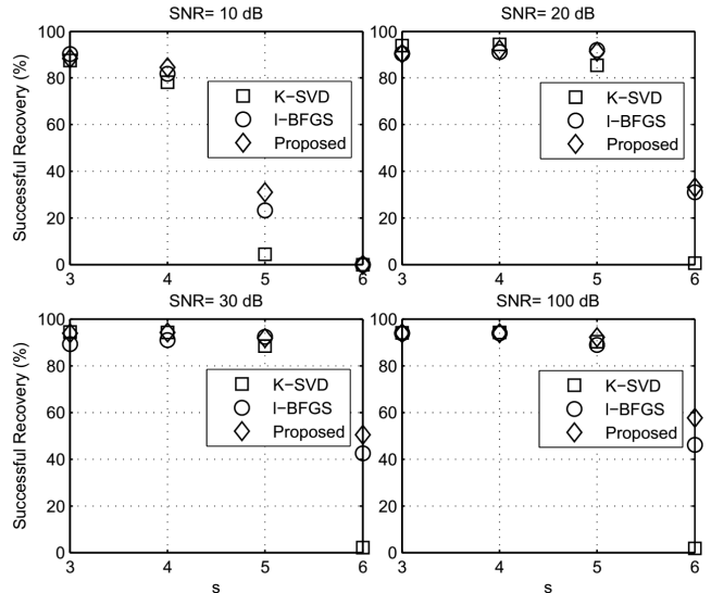
Fig. 1. Results of the experiment on synthetic data. Each figure corresponds to a certain noise level.
