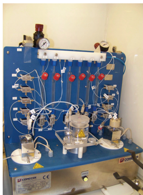
FIGURE 4: TADDEO module (COMECER, Castel Bolognese, Italy).
