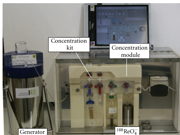
FIGURE 3: ^{188}\text{W}/^{188}\text{Re} generator and its remote-controlled elution/concentration system (IRE, Fleurus, Belgium).
