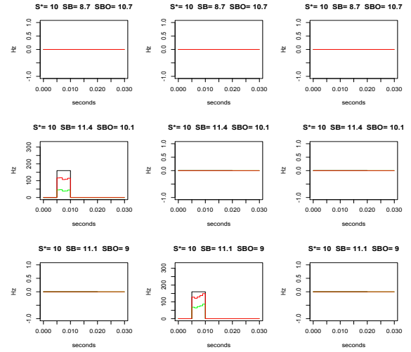
Fig. 4. Reconstructions of h_\ell^{(m)} ( \ell =column, m =row) for \ell, m = 1, 2, 3 by \tilde{f}_n in green (SB is the spontaneous rate estimate) and by \tilde{f}_n^{OLS} in red (SBO is the spontaneous rate estimate). The true f^* appears in black (S* is the true spontaneous rate).
