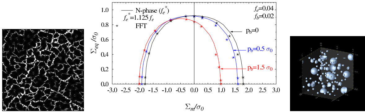
Figure 1: Left : 2D FFT simulation: localization of the local strain for an overall hydrostatic stress. Medium : Effective flow surfaces - 3D FFT simulations and model [1] ( f_e intergranular porosity, f_b intragranular local porosity, p_b and p_e intra and intergranular cavity pressures, \sigma_o yield stress of the sane matrix, \Sigma_m and \Sigma_{eq} overall hydrostatic and von Mises stresses, p_e = 0 ). Right : 3D unit cell.
