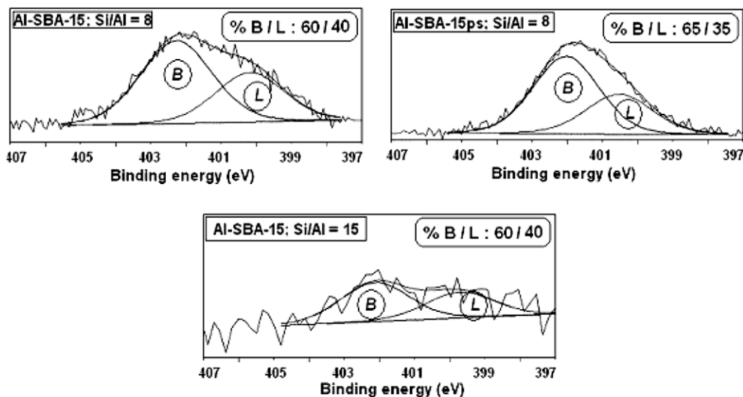
Fig. 8. N1s XP spectra after adsorption of \text{NH}_3 at 80 °C on three Al-SBA-15.
