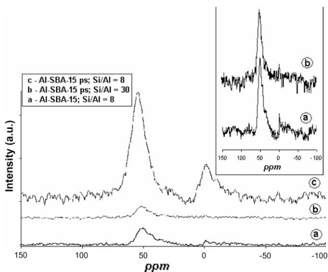
Fig. 3. ^{27}Al MAS NMR spectra of three Al-SBA-15 samples; Al-SBA-15 ( Si/Al_{gel} = 8 ); Al-SBA-15 ps ( Si/Al_{gel} = 30 ); Al-SBA-15ps ( Si/Al_{gel} = 8 ).
