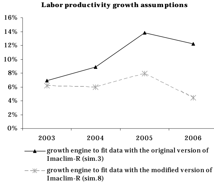
Figure 7: Mean labor productivity growth assumptions to fit GDP data with the original version of the model (simulation 3) (black triangles) and with the modified version of the model (simulation 8) (grey crosses).
