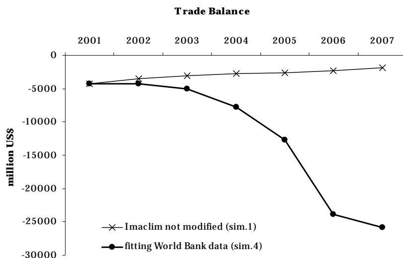
Figure 4: Indian trade balance between 2001 and 2007, as modeled by the original version of the model (crosses) and as observed by the World Bank (points). In the modified model version, the trade balance is forced to follow the observations (simulation 4).
