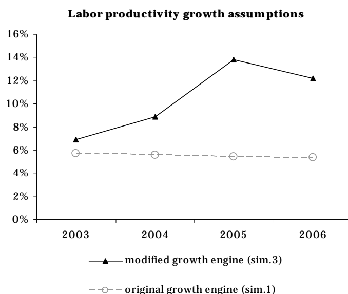
Figure 2: Mean labor productivity growth assumptions, for the original model (simulation 1) (grey dots) and for the modified (black triangles) growth engine, such that the model reproduces observed GDP over the 2003-2006 period (simulation 3).
