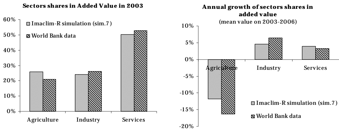
Figure 6: Sectors shares in Added Value in 2003 and their mean annual growth rate over the 2003-2006 period, as modeled (results from simulation 7) and in the World Bank data 6 .
