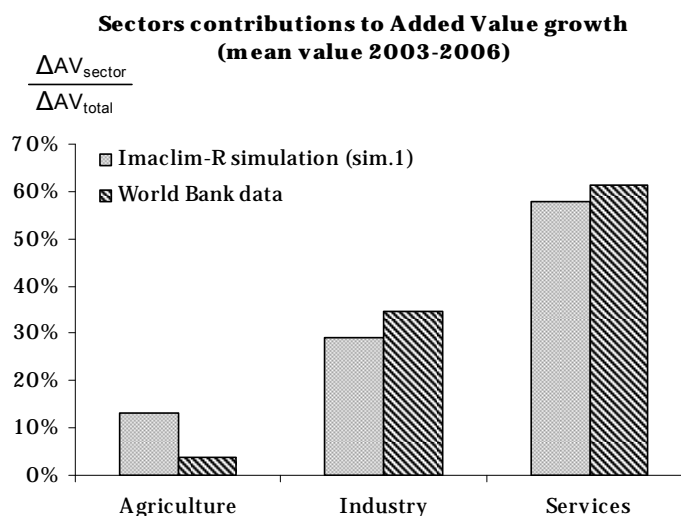
Figure 3: Sectors contribution to Added Value growth the 2003-2006 period, as modeled (results from simulation 1) and in the World Bank data 6 .
