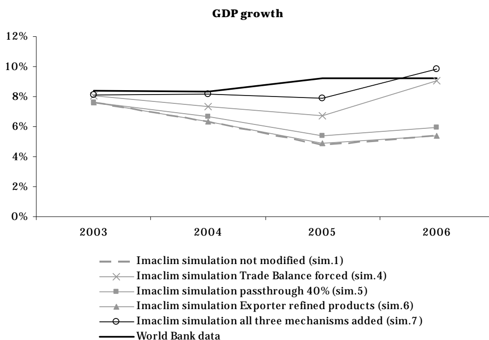
Figure 5: Observed GDP growth in India between 2003 and 2006, and results of the initial model version (simulation 1) and of several modified model versions, including one (simulations 4, 5 and 6) or all additional short-term mechanisms (simulation 7).
