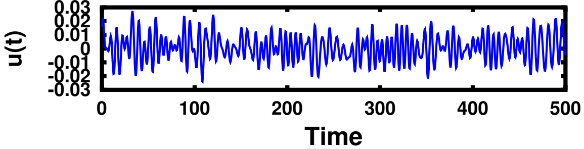
Figure 1: The control that drives \psi_0 to \psi_T (cf. equation (8)) irrespective of the perturbation \alpha_k \in \{-0.1, 0, 0.1\} . The quality of the control is over 99% for any perturbation. However the trajectories \psi(t) corresponding to u(t) - 0.1 , u(t) and u(t) + 0.1 are all different.
